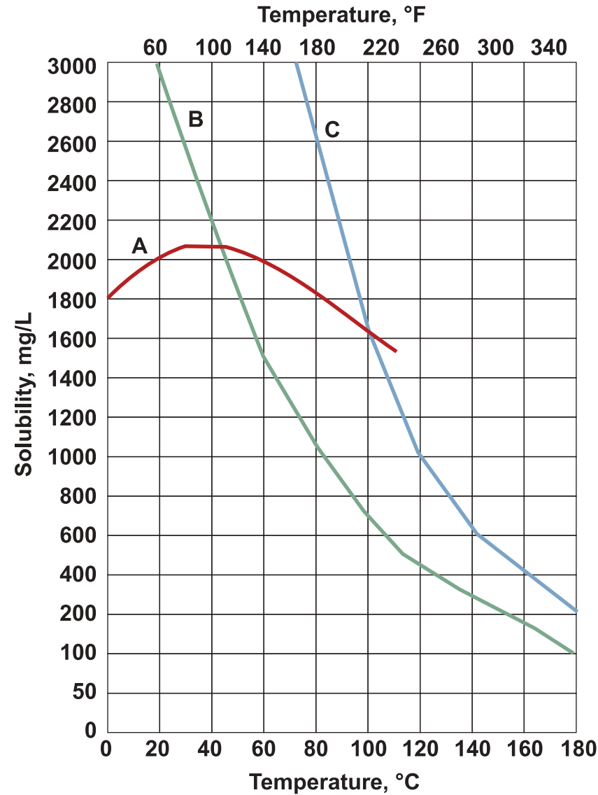
Figure 8.3. Solubility of three forms of calcium sulfate ( \text{CaSO}_4 ) versus water temperature: A) \text{CaSO}_4 \cdot 2\text{H}_2\text{O} , B) Anhydrous \text{CaSO}_4 , C) Hemihydrate \text{CaSO}_4 \cdot \frac{1}{2}\text{H}_2\text{O} .
