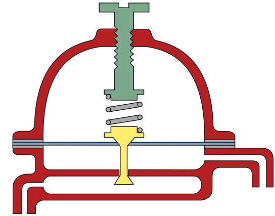
Figure 4.12 The automatic expansion valve (constant pressure valve).
