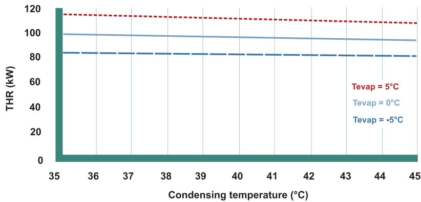
Figure 3.8 How change in evaporation temperature and condensation temperature affect the total heat of rejection for a specific compressor type.
