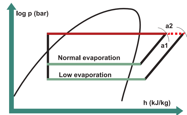
Figure 10.15 A log P/h diagram showing the resulting higher discharge temperature for a larger compression step.
