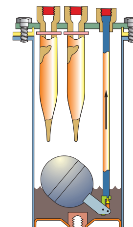
Figure 2.13 Oil separator.
