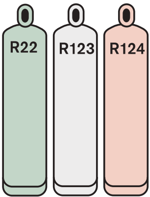
Figure 5.3 Some HCFC refrigerants.
