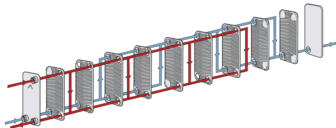
Figure 1.12 Two-pass over one-pass configuration.
