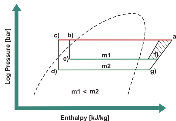
Figure 10.13 An economizer system (right) and a log P/h diagram (above). The refrigerant flow is divided after point (b). The smaller flow (m1) is evaporated at an intermediate pressure to cool the main flow (m2). The cold intermediate gas (f) enters the compressor in a special economizer port.
