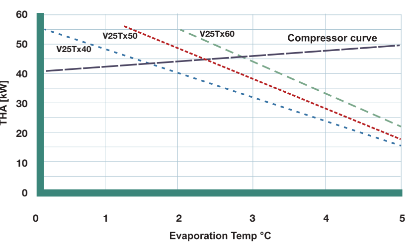
Figure 6.25 Different operating points for different evaporators operating with the same compressor.
