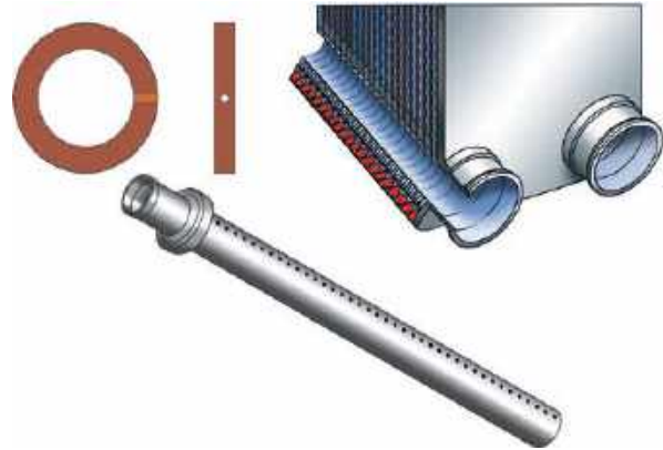
Figure 6.18 SWEP distribution devices.
