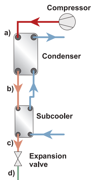
Figure 10.12 Schematic design of a condenser and a separate subcooler with a shared secondary fluid stream.
