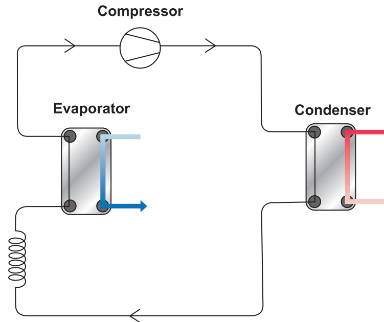
Figure 4.11 The refrigerant cycle with a capillary tube installed.
