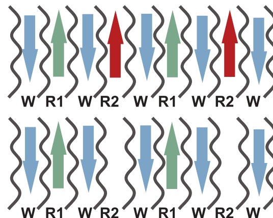
Figure 6.30 The flow channels through a True Dual BPHE. The upper figure shows a BPHE running on full load and the lower flow channels show a BPHE running on half load (one refrigerant circuit is closed).
