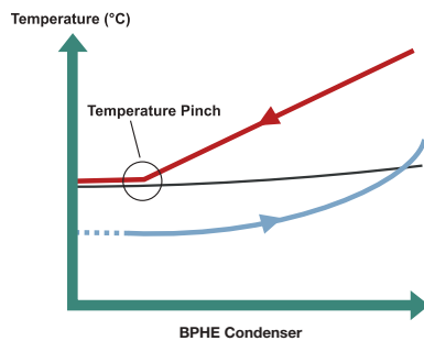
Figure 7.22 A temperature program inside a BPHE condenser with a low secondary flow is compared with a BPHE desuperheater. The similar temperatures in the condenser reduce the heat transfer. In contrast, the pinch is avoided in a desuperheater and the heat transfer remains efficient.
