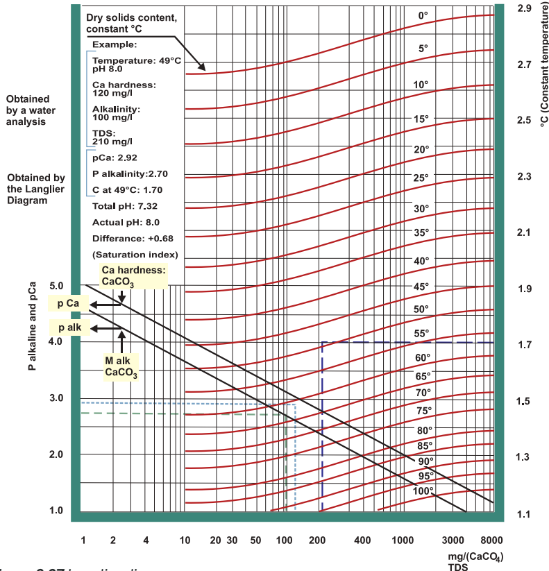
Figure 8.37 Langlier diagram.
