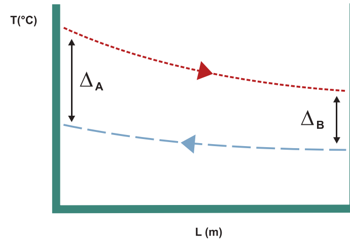
Figure 1.6 The temperature program for calculation of LMTD.
