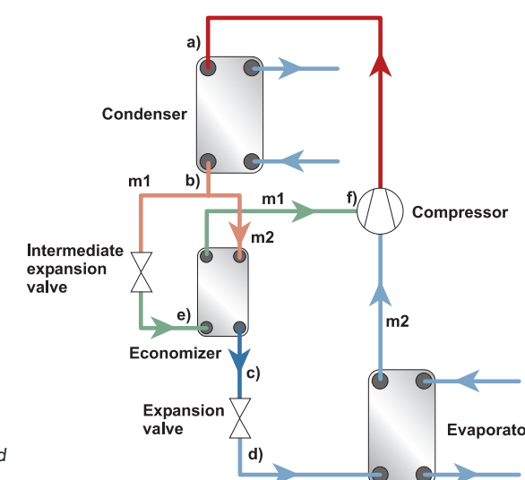
Figure 10.13 An economizer system (right) and a log P/h diagram (above). The refrigerant flow is divided after point (b). The smaller flow (m1) is evaporated at an intermediate pressure to cool the main flow (m2). The cold intermediate gas (f) enters the compressor in a special economizer port.
