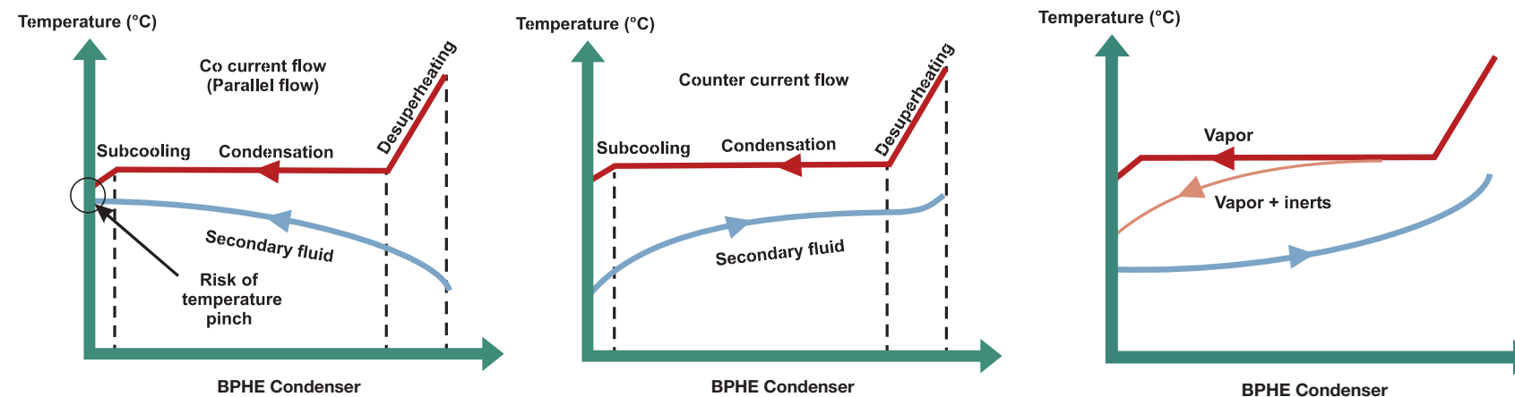
Figure 7.5 Temperature profiles for co-current and counter-current condensers.
