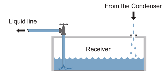
Figure 2.14 Liquid receiver.
