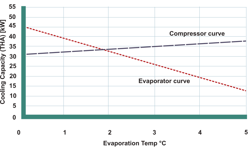
Figure 6.24 Evaporator curve vs. compressor curve. The operating point is found where the two curves meet.
