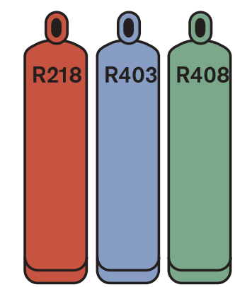
Figure 5.5 Some fluorocarbon refrigerants.
